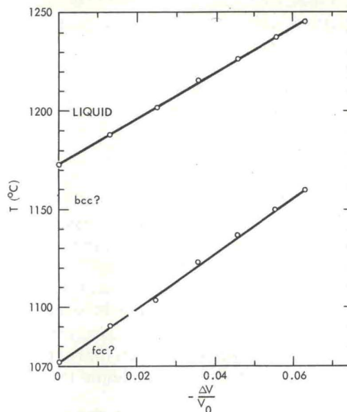
Fig. 5. Transition temperatures vs. compression for americium.
