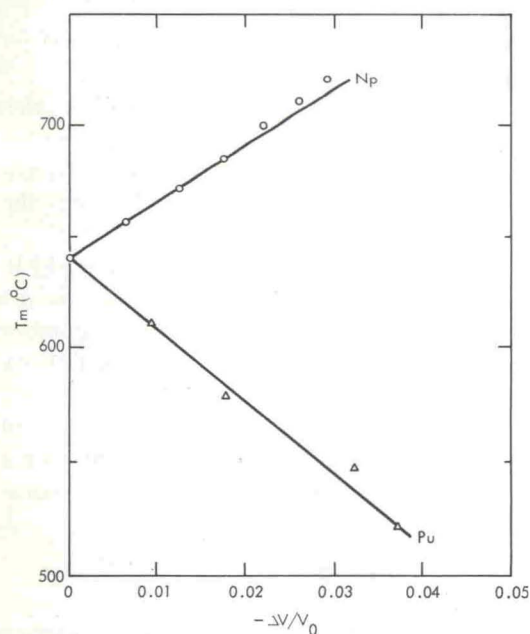
Fig. 6. Melting curves vs. compression for neptunium and plutonium.
