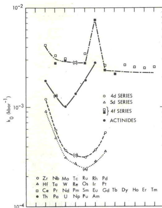
Fig. 4. Comparison of compressibilities for transition metals, rare earths, and actinides.
