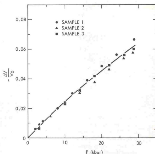
Fig. 1. Compression of americium vs. pressure.
