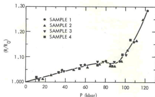
Fig. 3. Resistance of americium vs. pressure.
