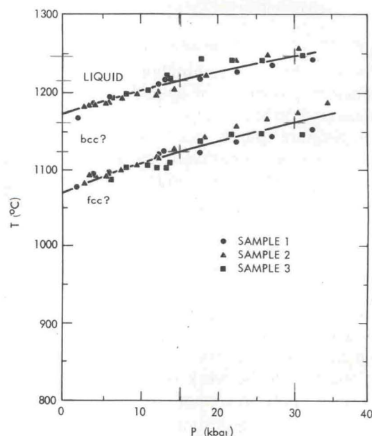
Fig. 2. Phase diagram of americium.
